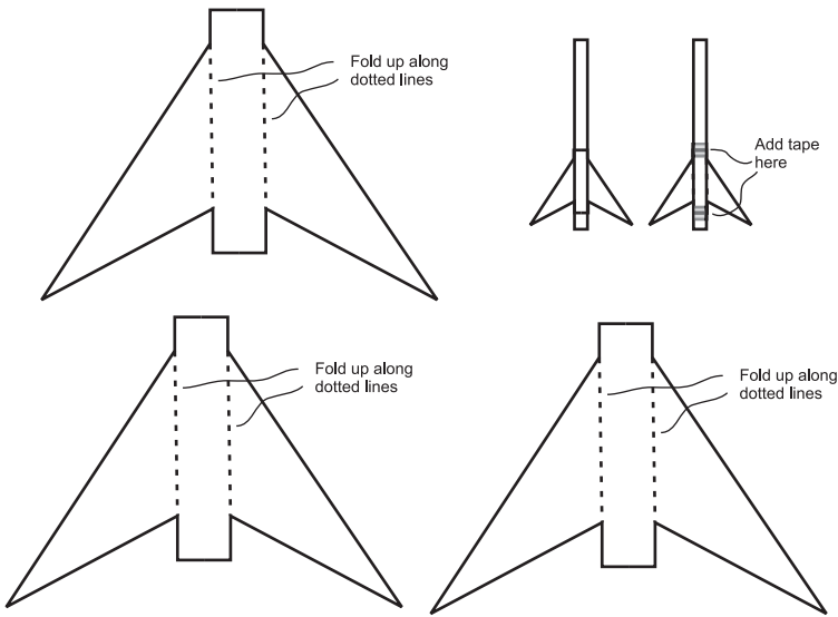
Fin Pattern: Two patterns = 4 fins per rocket
